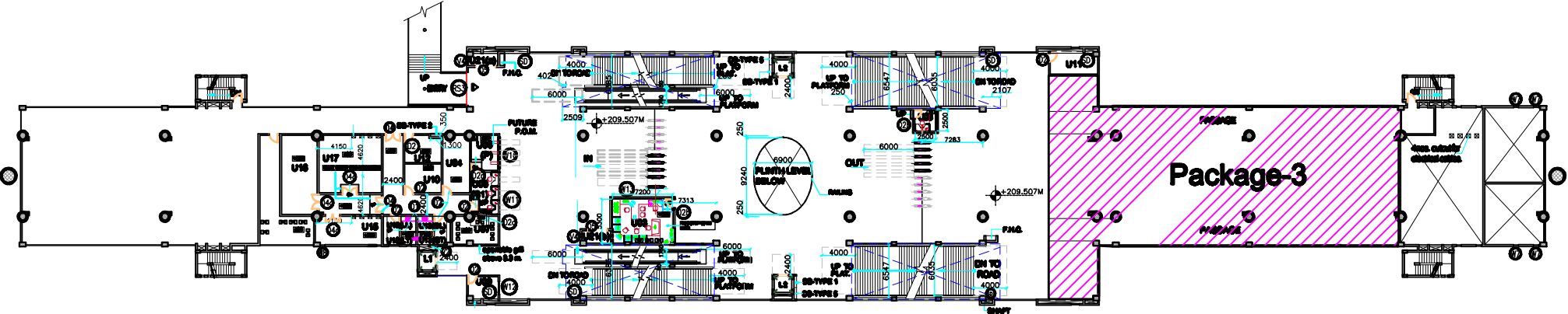
JHILMIL METRO STATION (Package-3) - Concourse Level Plan
